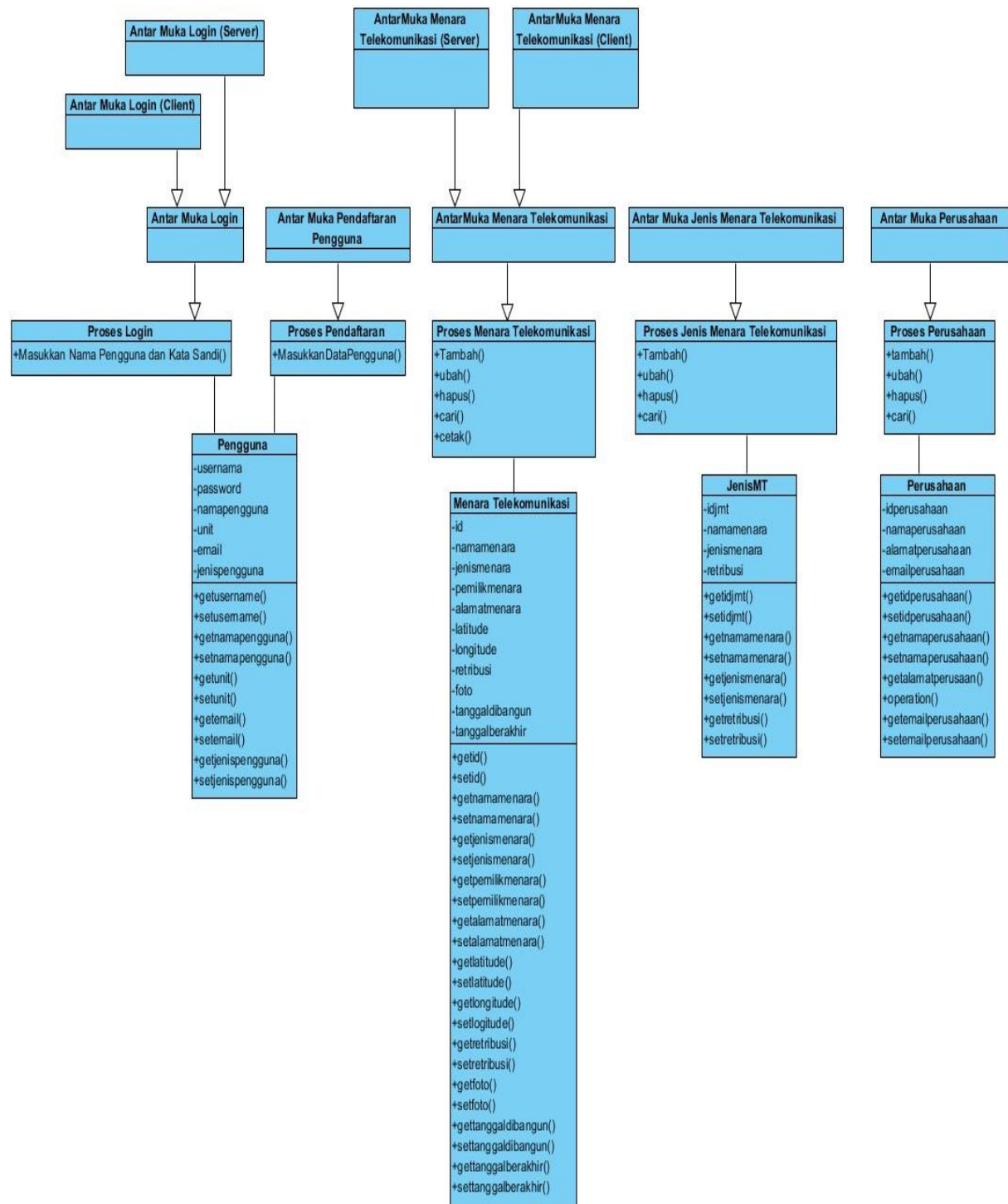
Gambar 5. Class Diagram
