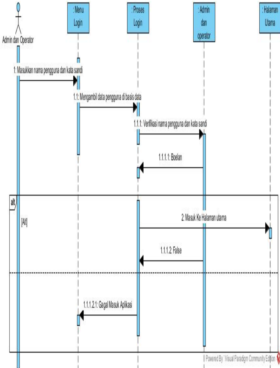
Gambar 4. Sequence Diagram
