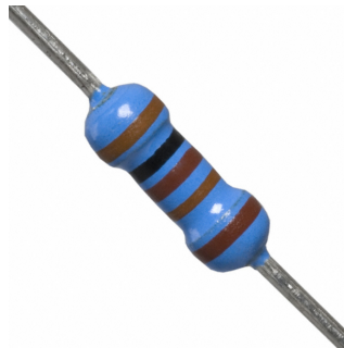
Figure 7. Resistor 301k
